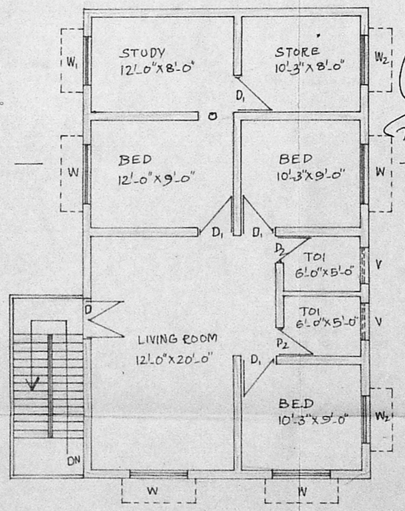
SECOND FLOOR PLAN (PRO)
