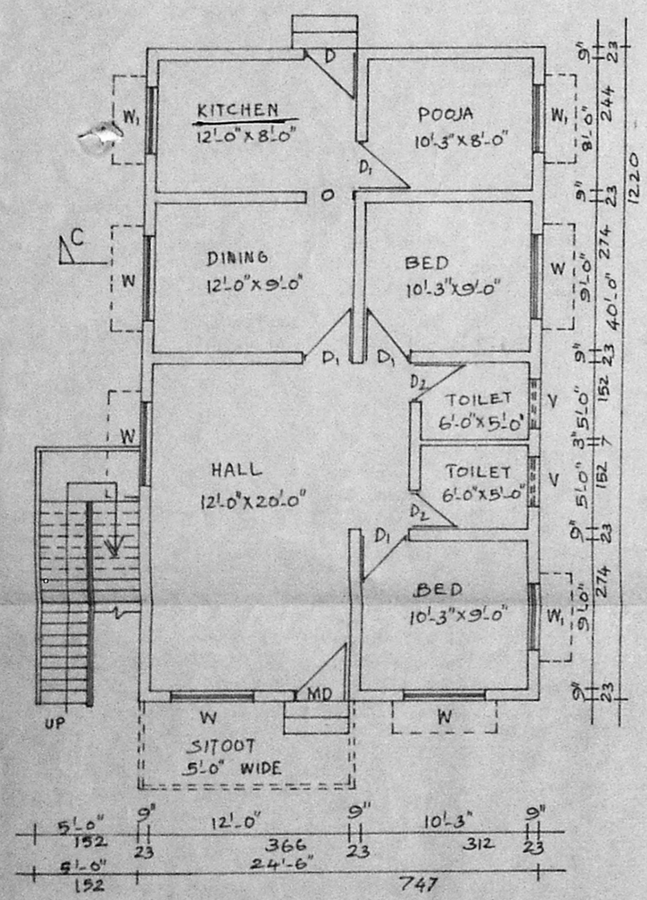
DETAILS OF GROUND FLOOR PLAN (EXT)
