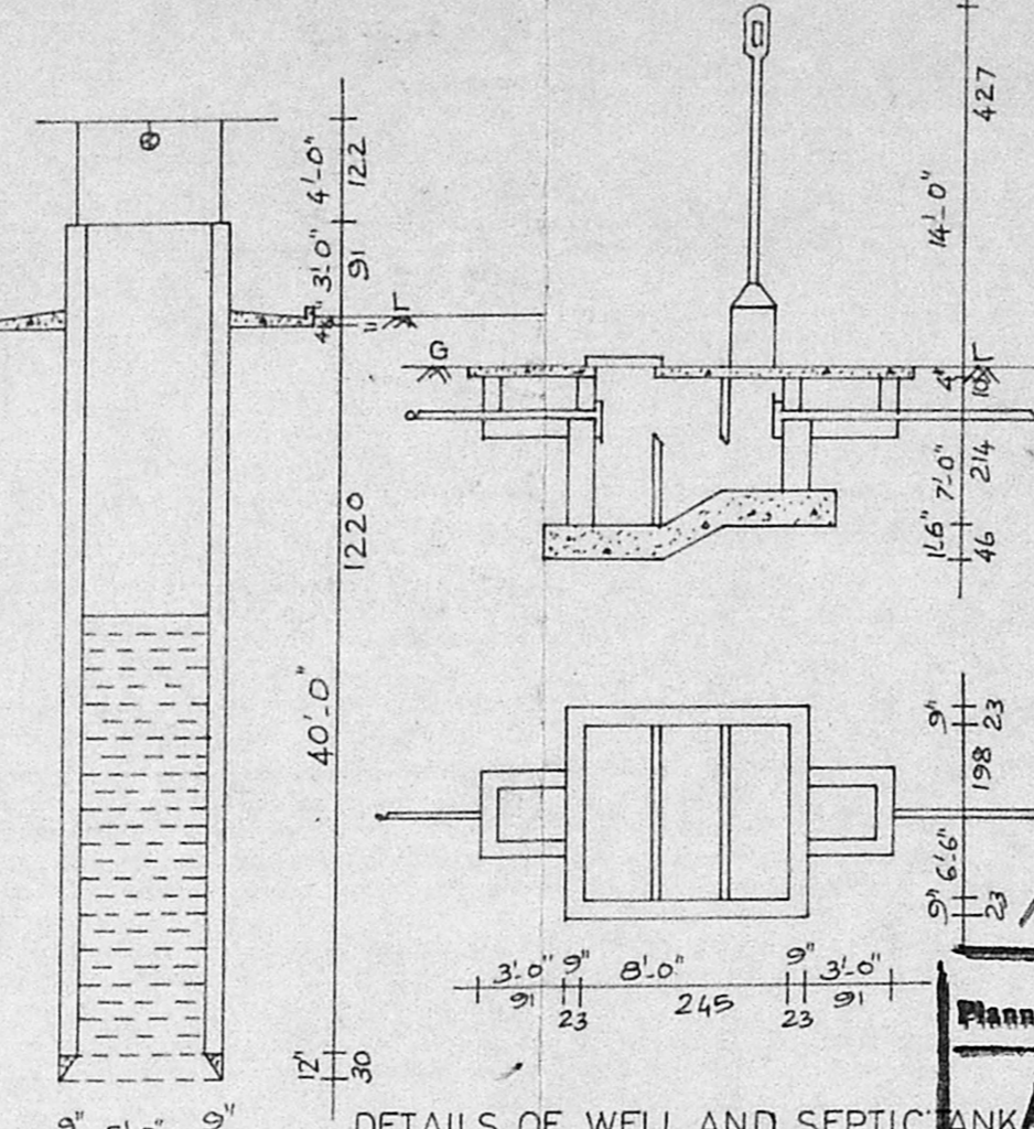
DETAILS OF WELL AND SEPTIC TANK
