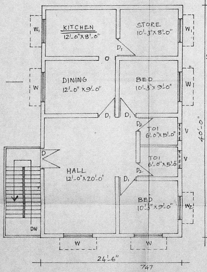
FIRST FLOOR PLAN (EXT)
