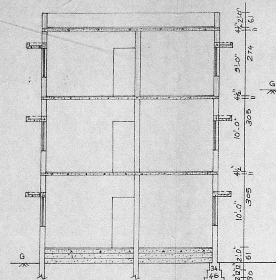
SECTION ON CD
